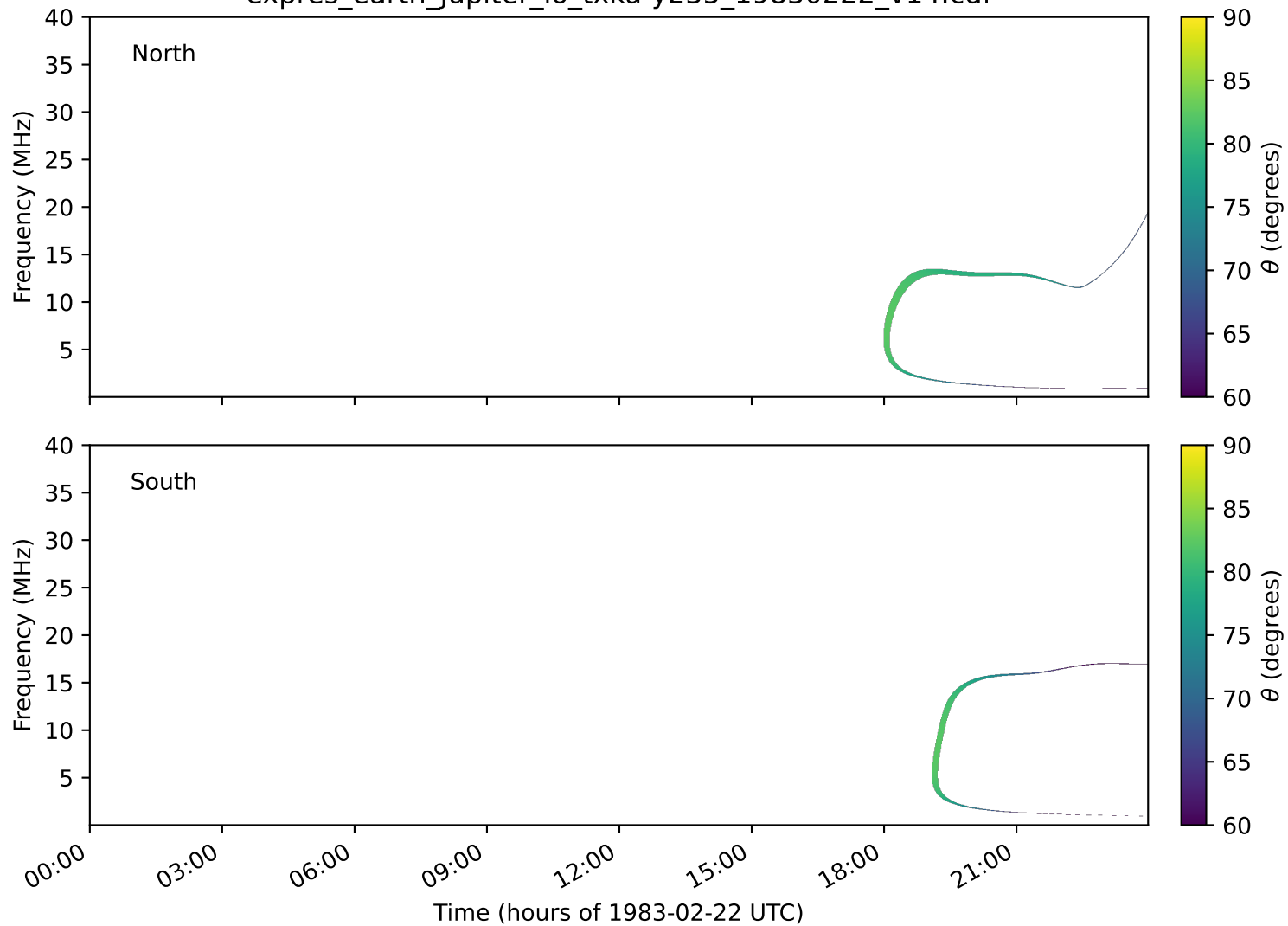
expres_earth_jupiter_io_txka-y235_19830222_v14.cdf
