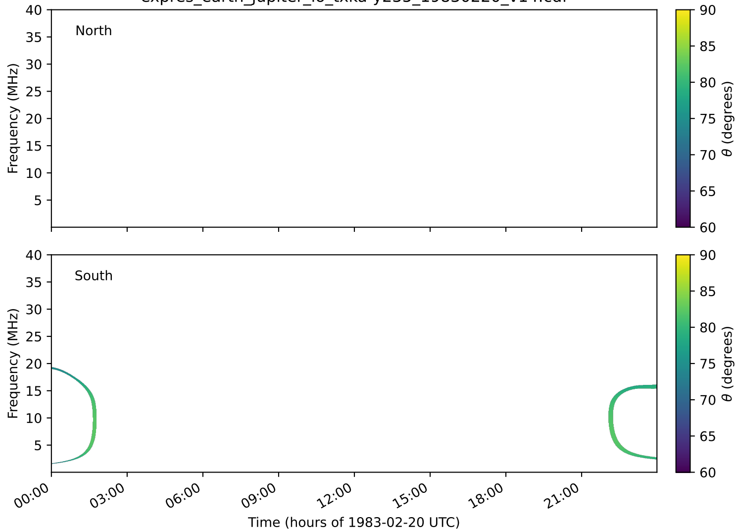
expres_earth_jupiter_io_txka-y235_19830220_v14.cdf
