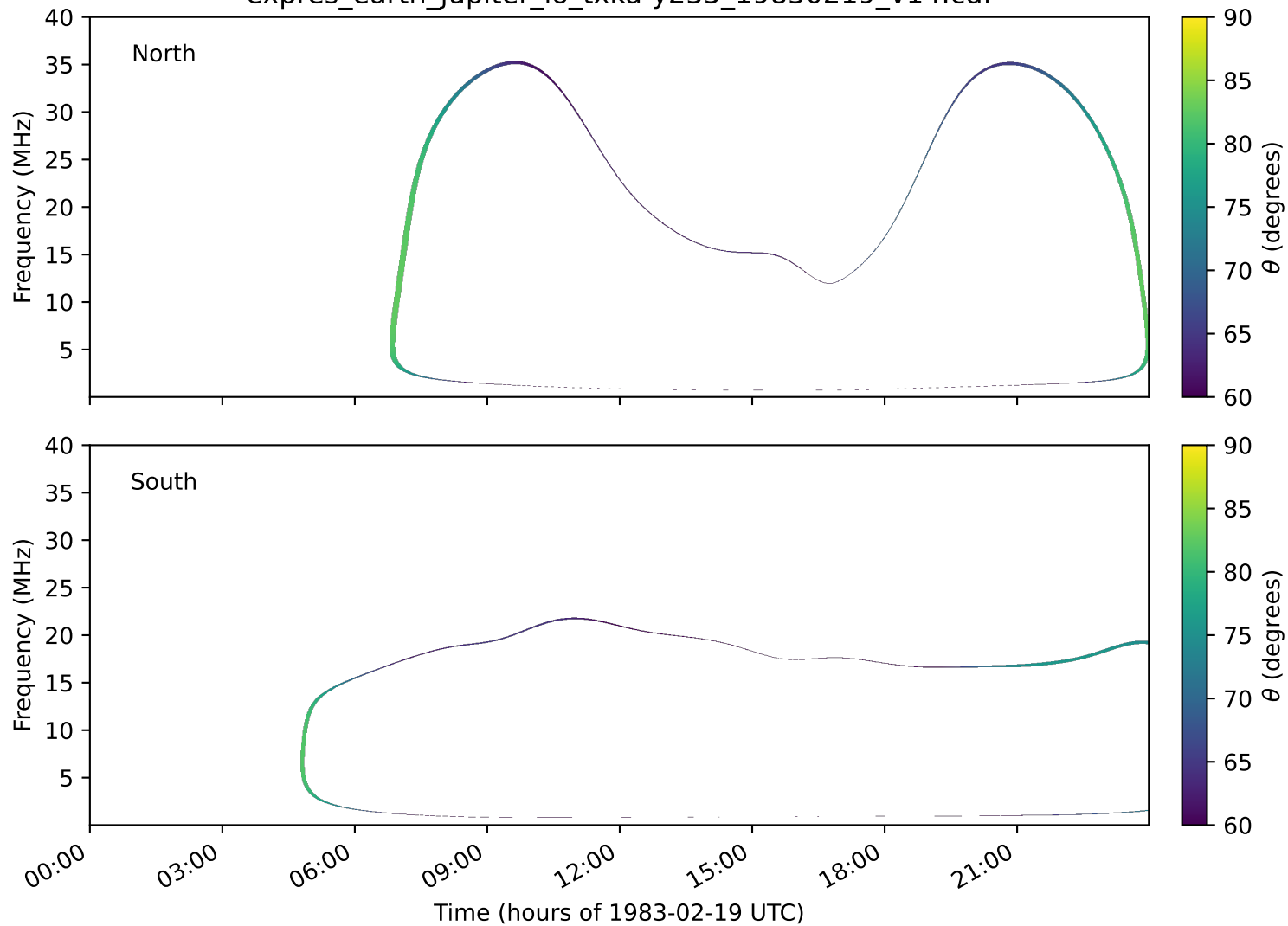
expres_earth_jupiter_io_txka-y235_19830219_v14.cdf
