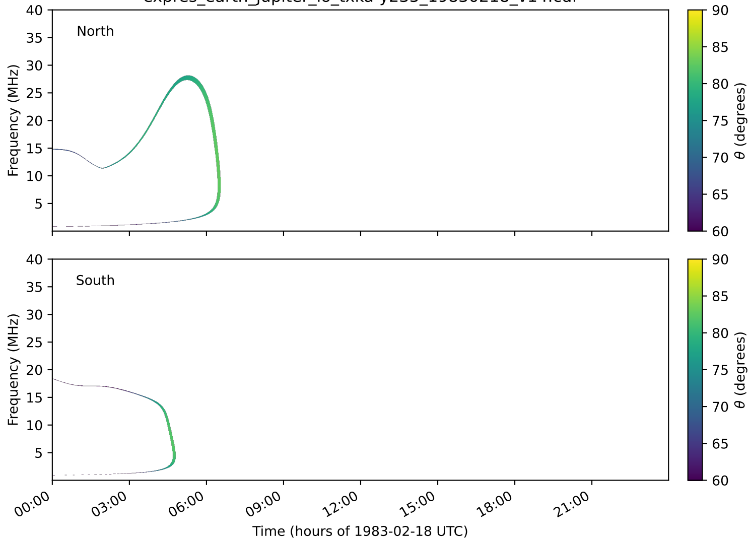
expres_earth_jupiter_io_txka-y235_19830218_v14.cdf
