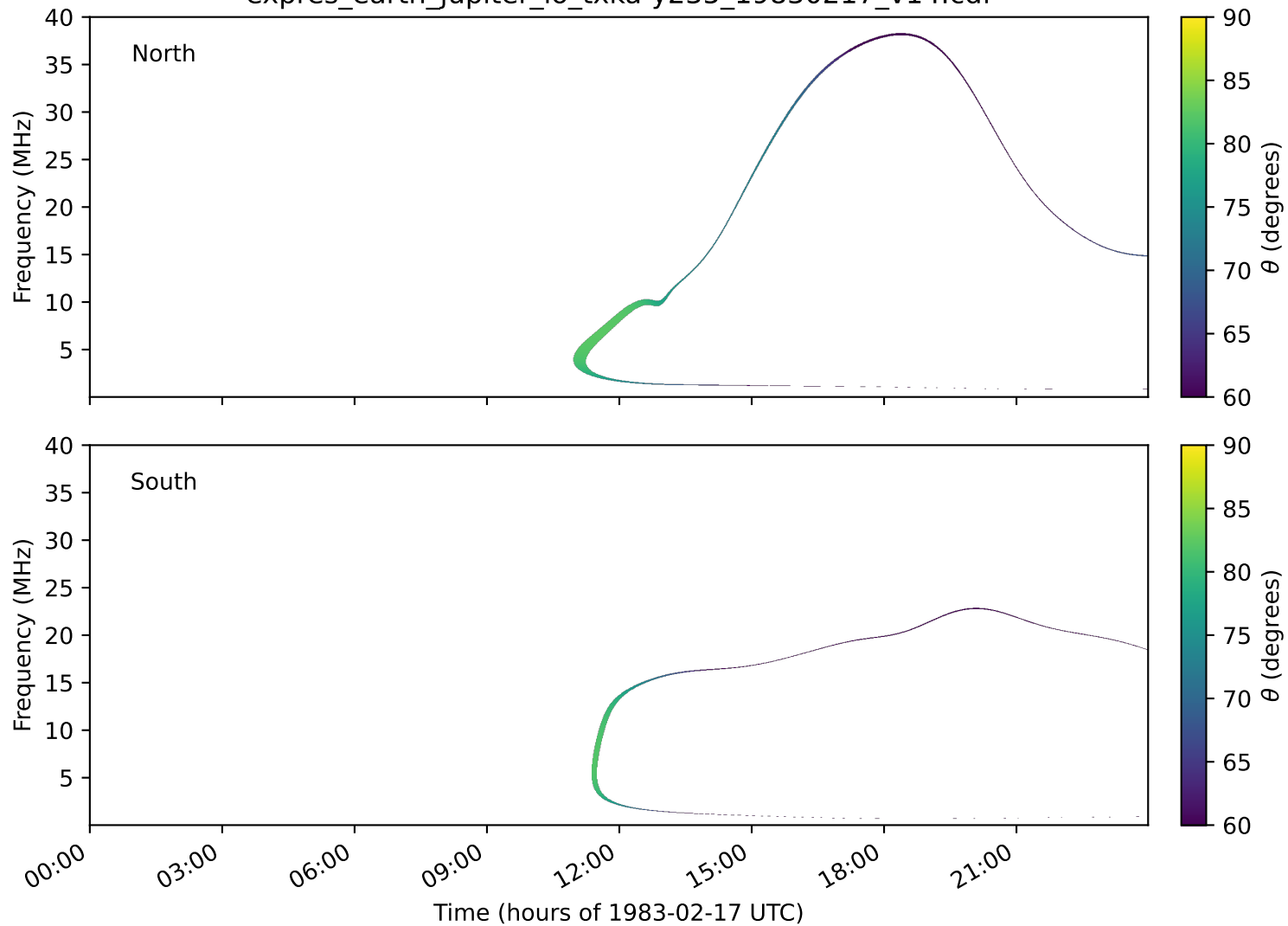
expres_earth_jupiter_io_txka-y235_19830217_v14.cdf
