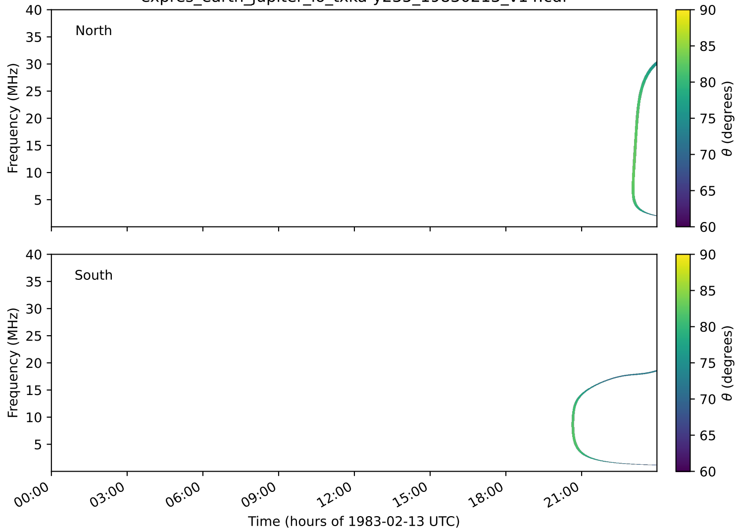
expres_earth_jupiter_io_txka-y235_19830213_v14.cdf
