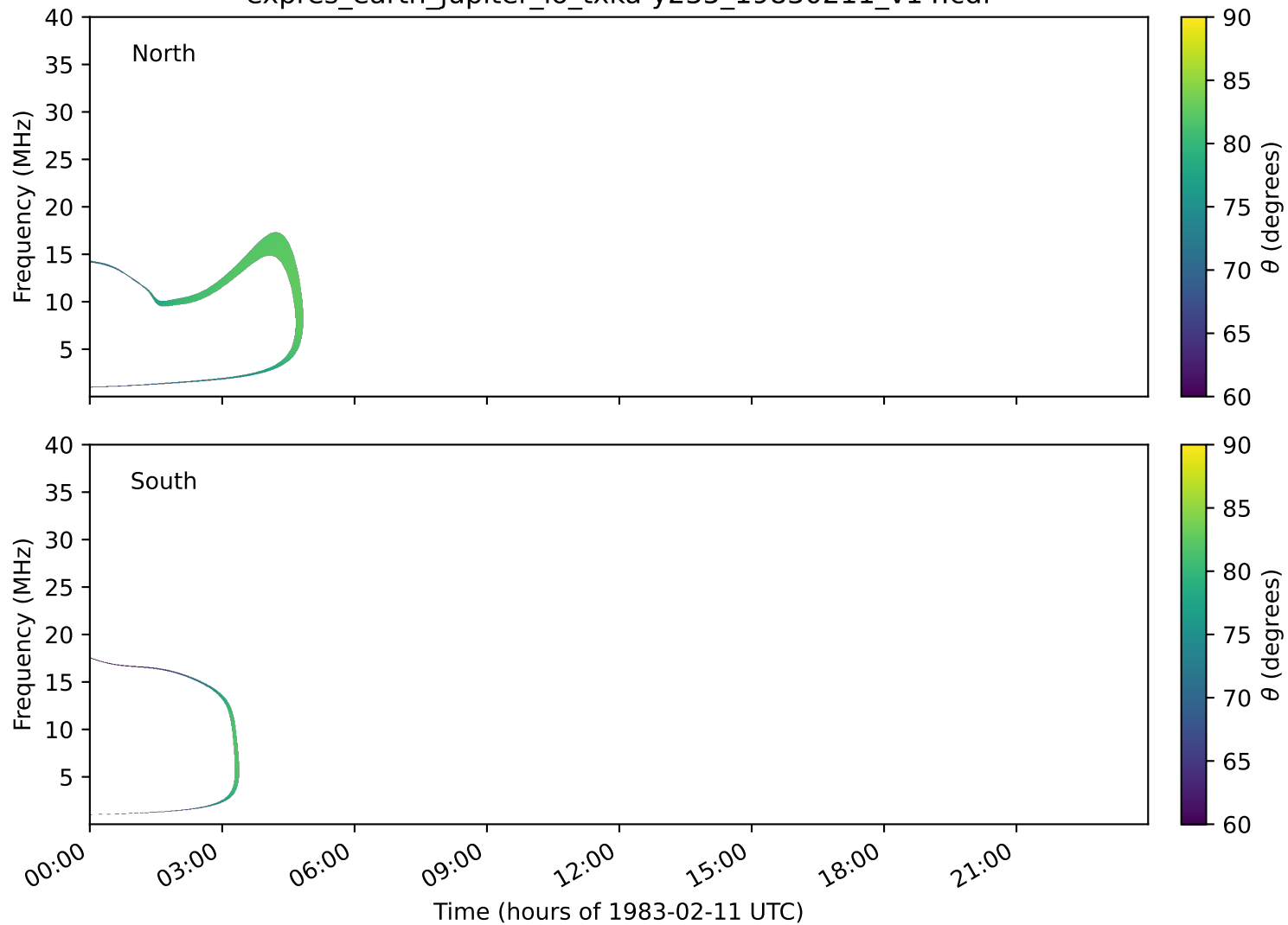
expres_earth_jupiter_io_txka-y235_19830211_v14.cdf
