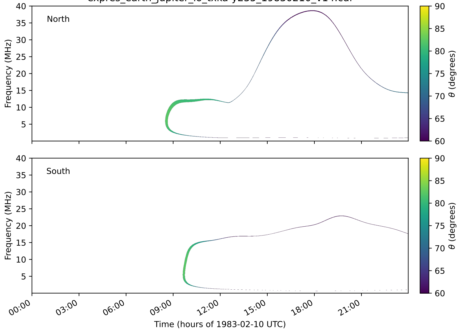
expres_earth_jupiter_io_txka-y235_19830210_v14.cdf
