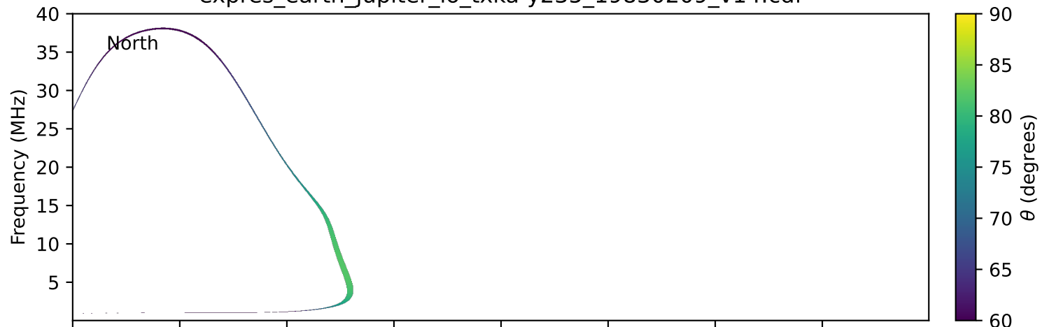
expres_earth_jupiter_io_txka-y235_19830209_v14.cdf
