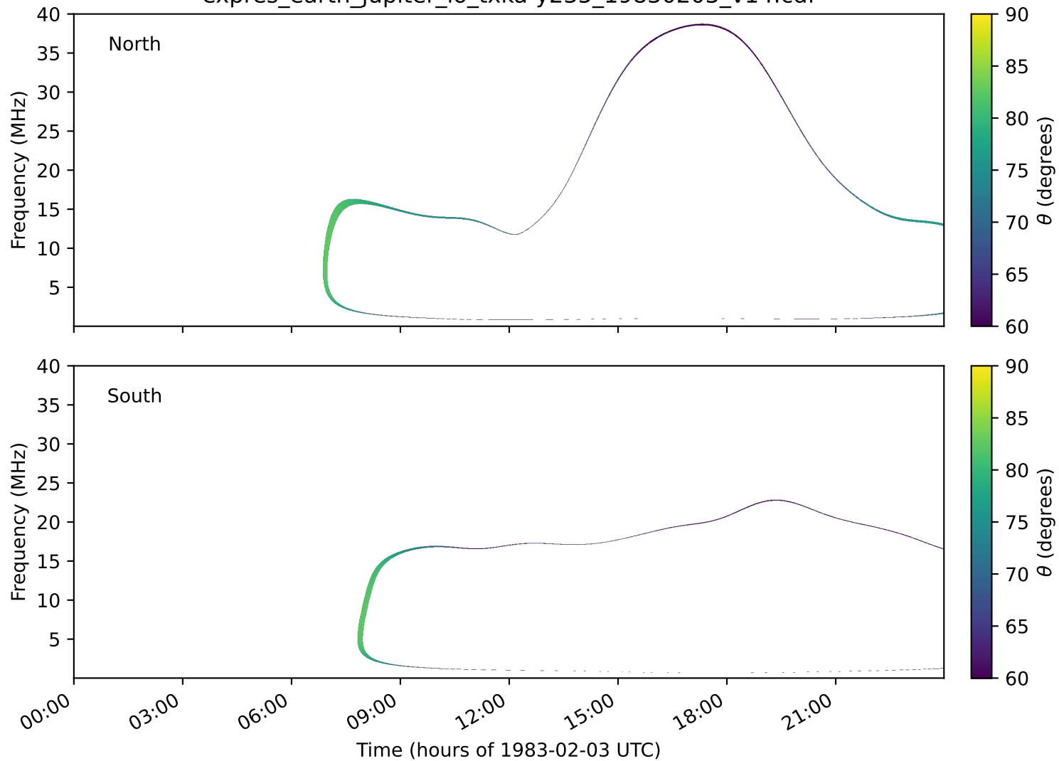
expres_earth_jupiter_io_txka-y235_19830203_v14.cdf
