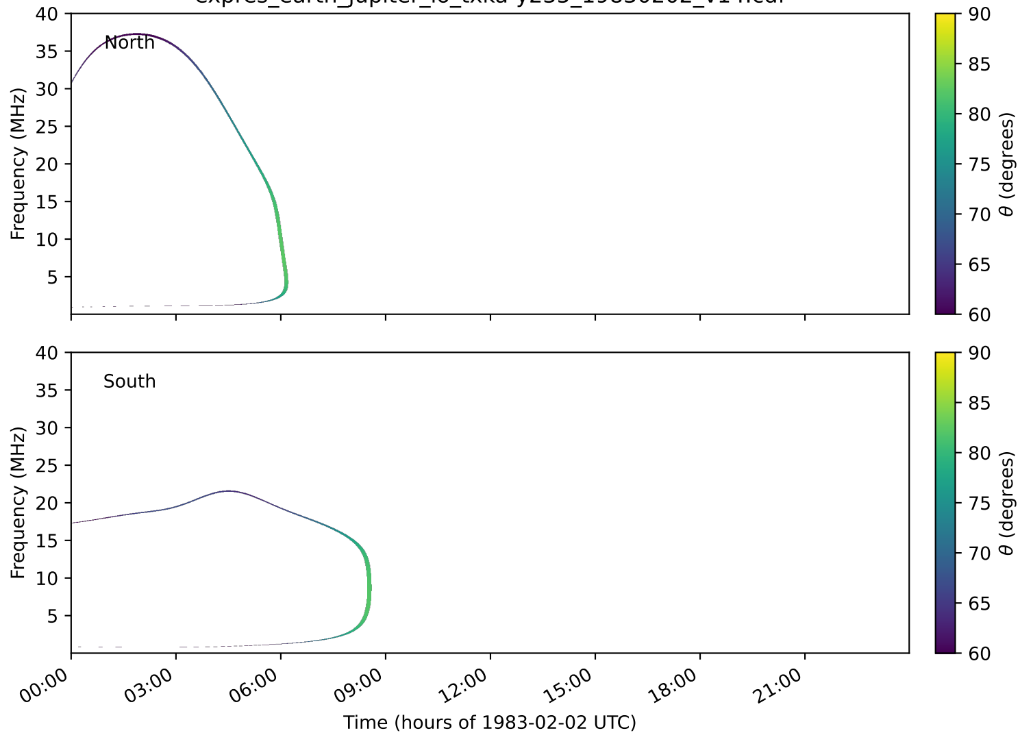
expres_earth_jupiter_io_txka-y235_19830202_v14.cdf
