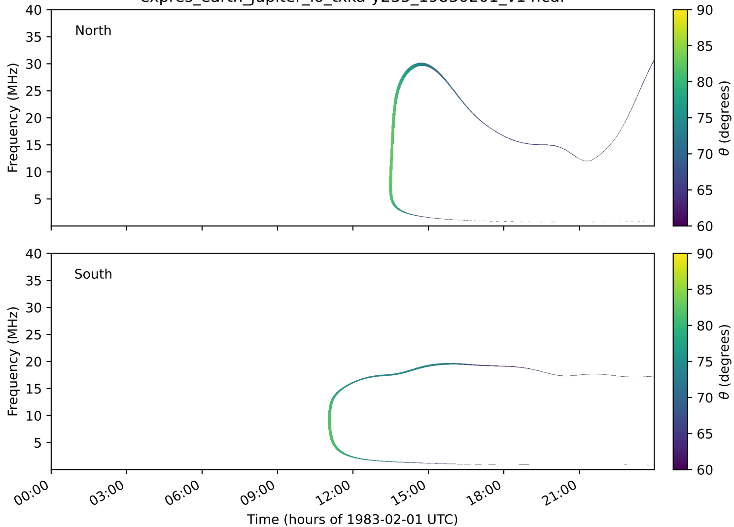
expres_earth_jupiter_io_txka-y235_19830201_v14.cdf
