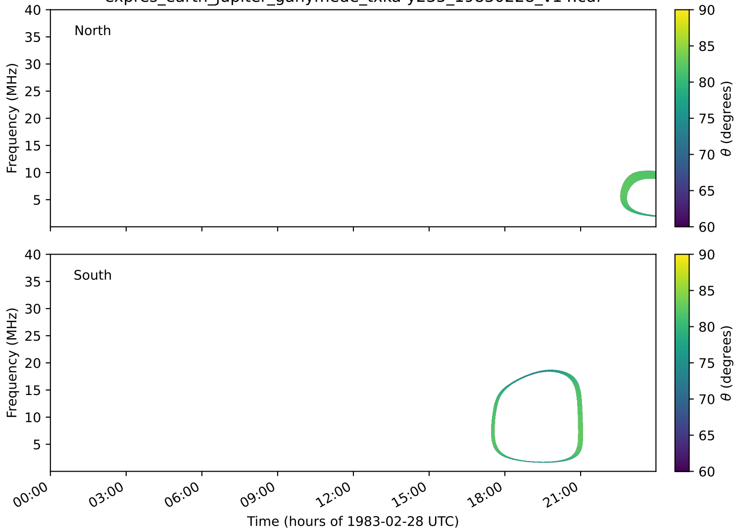
expres_earth_jupiter_ganymede_txka-y235_19830228_v14.cdf
