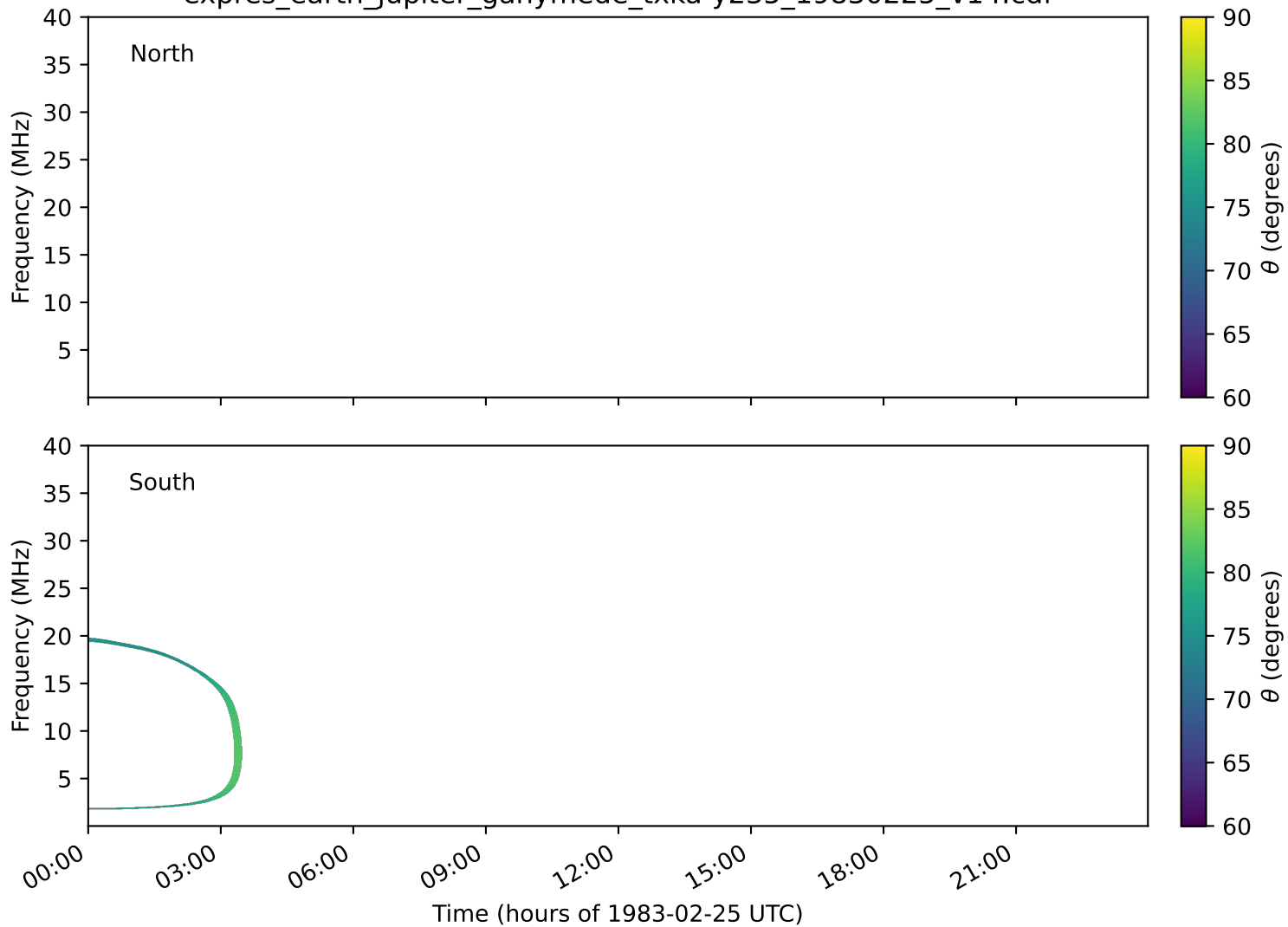
expres_earth_jupiter_ganymede_txka-y235_19830225_v14.cdf
