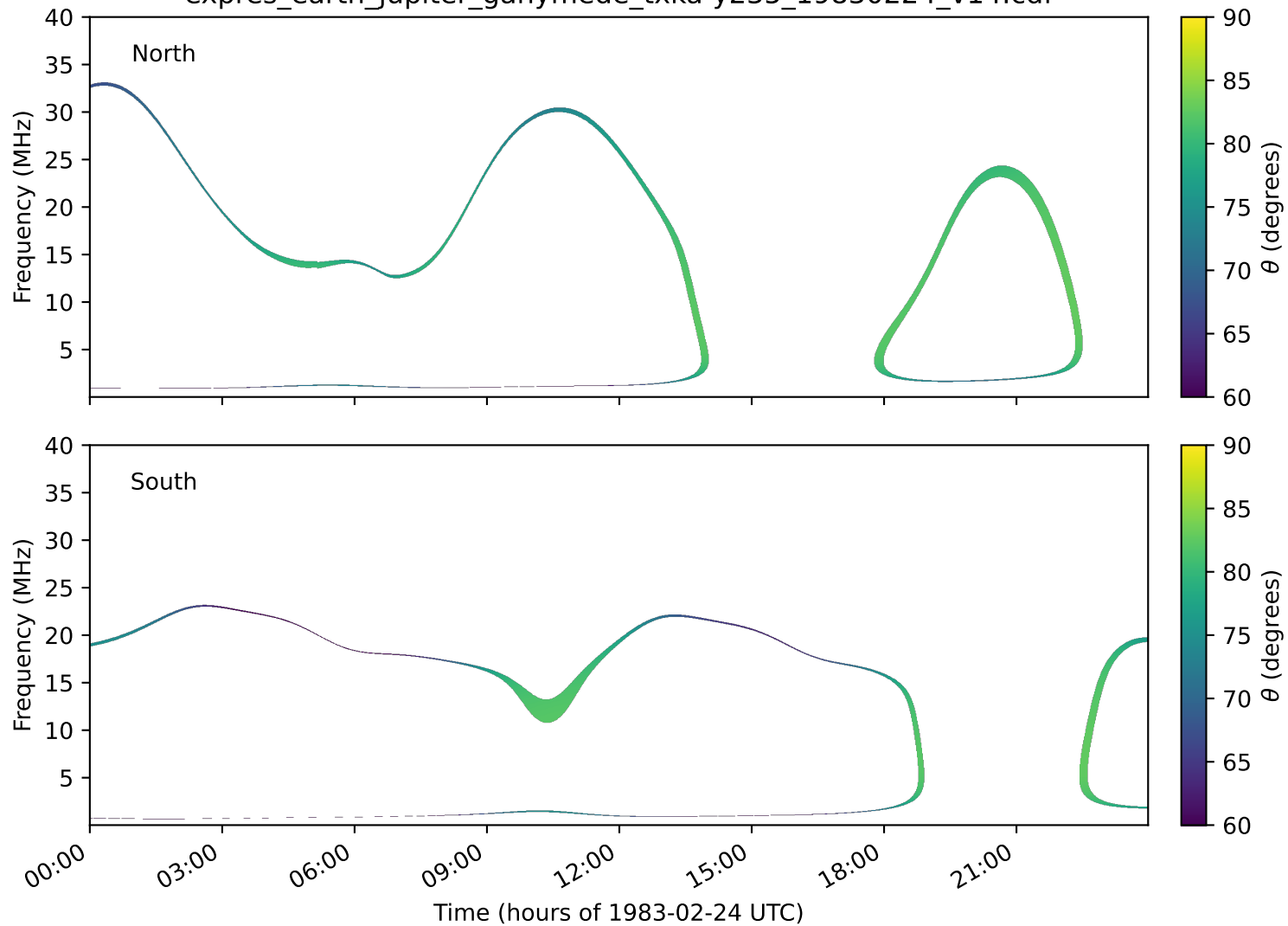
expres_earth_jupiter_ganymede_txka-y235_19830224_v14.cdf
