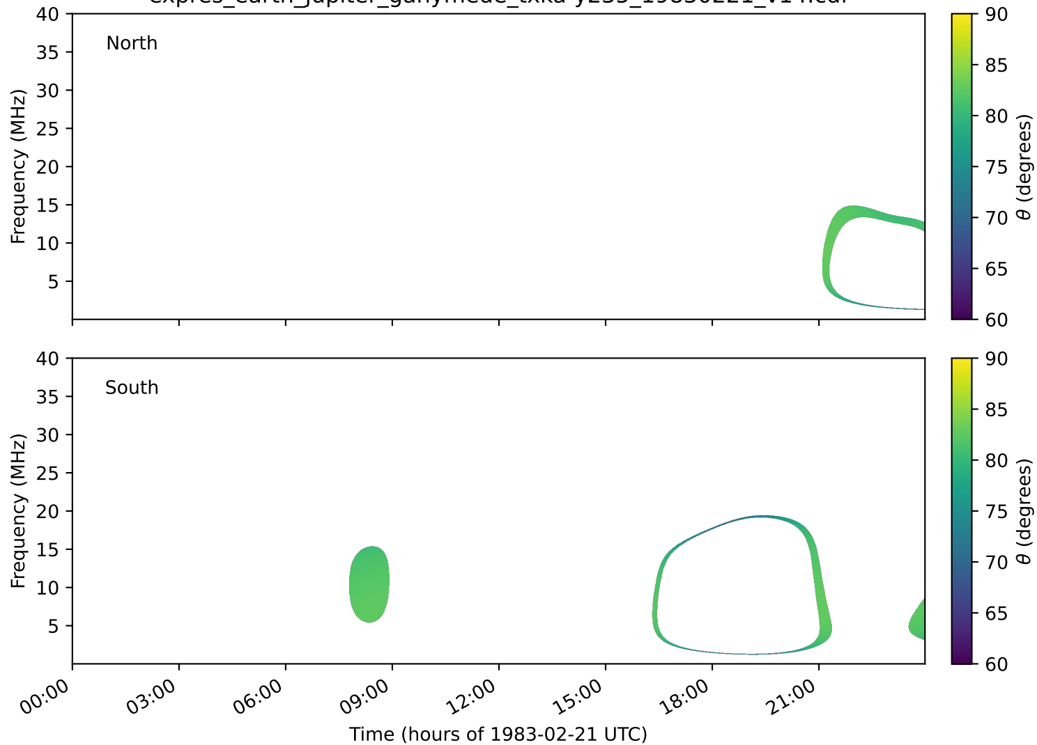
expres_earth_jupiter_ganymede_txka-y235_19830221_v14.cdf
