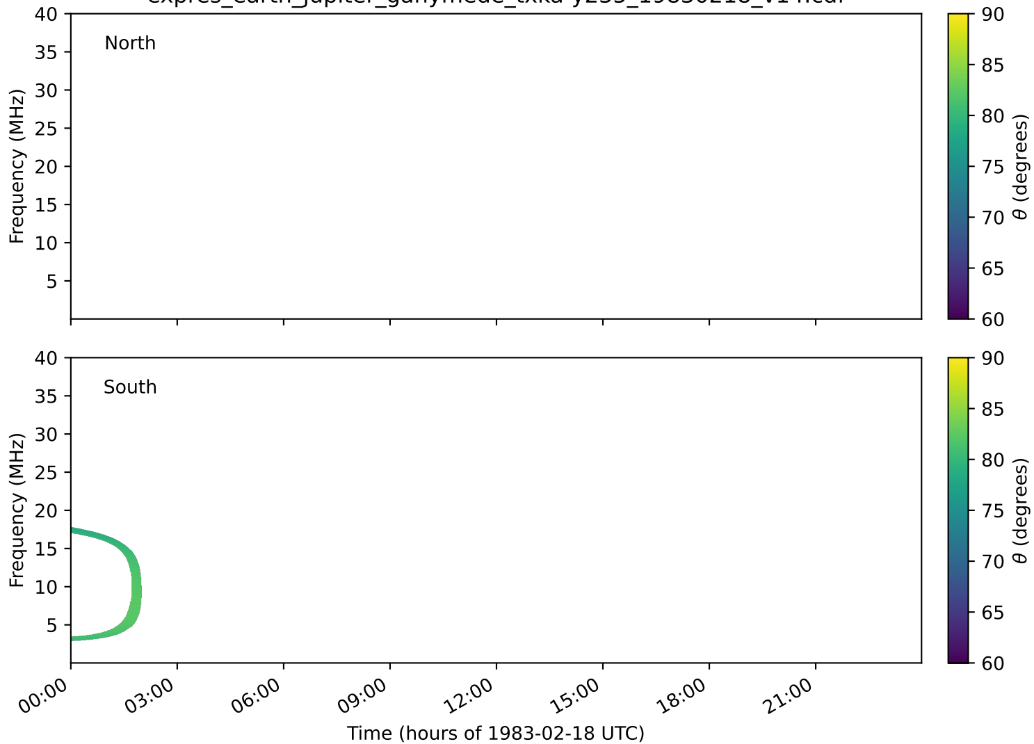
expres_earth_jupiter_ganymede_txka-y235_19830218_v14.cdf
