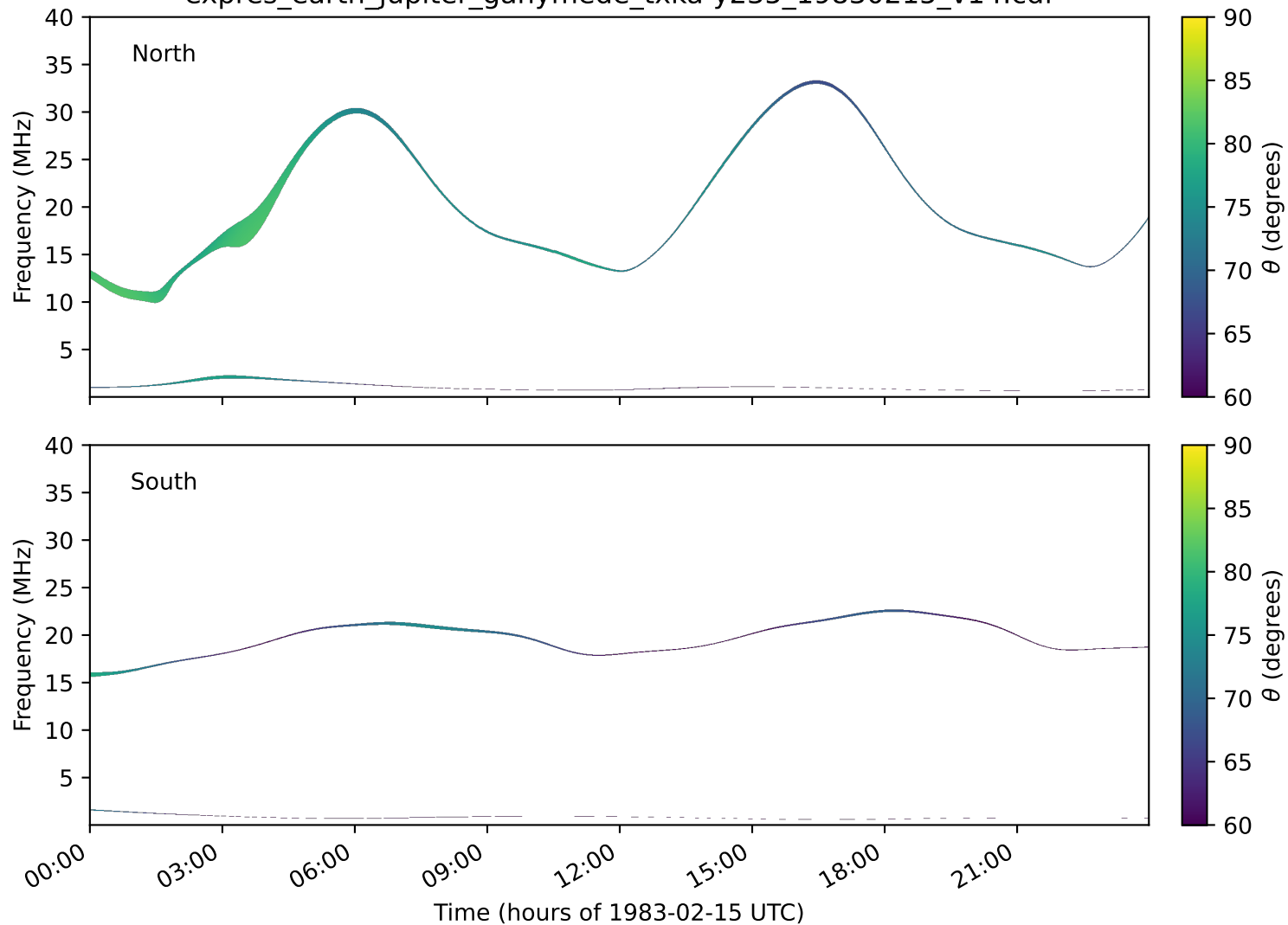
expres_earth_jupiter_ganymede_txka-y235_19830215_v14.cdf
