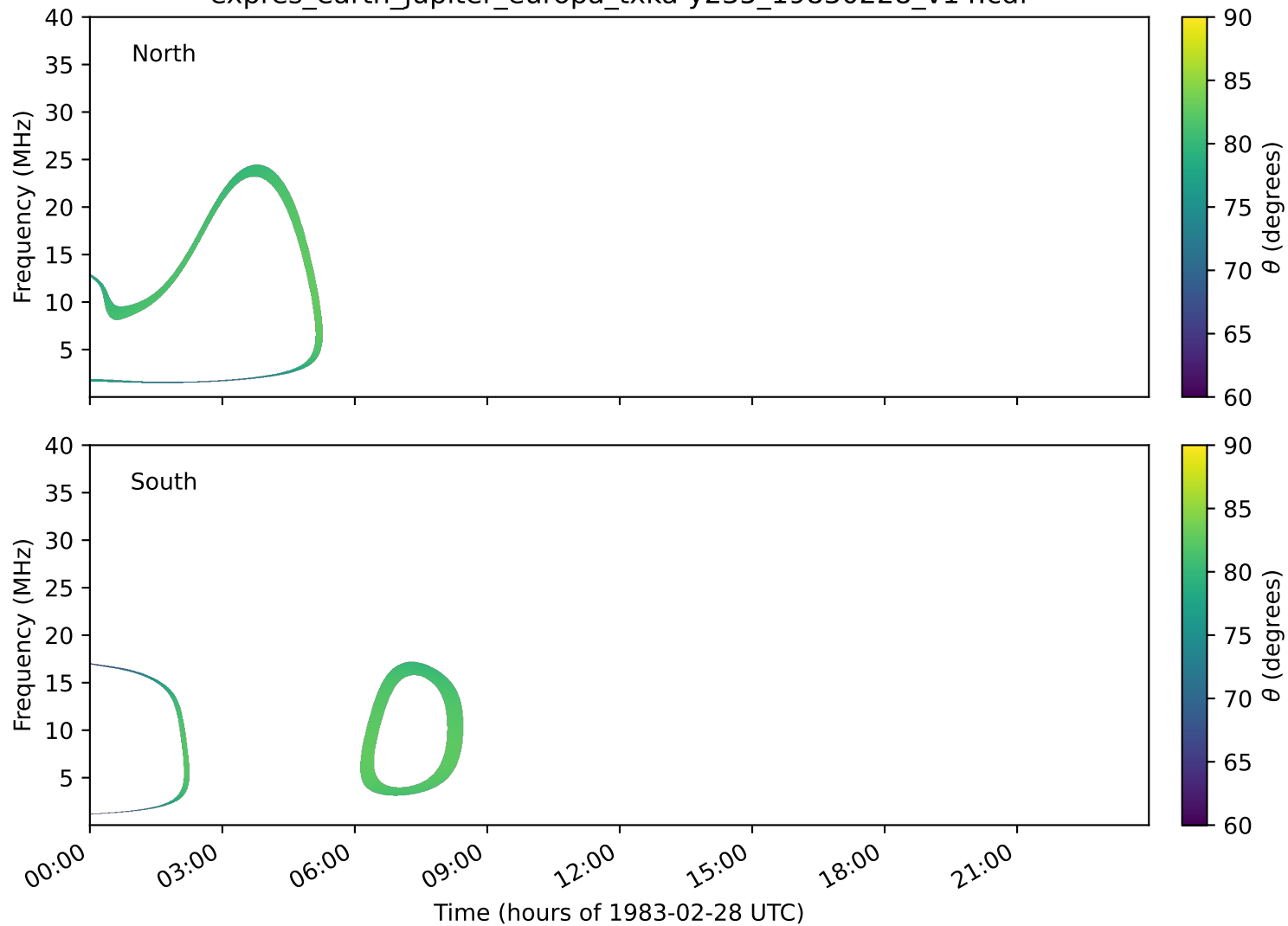
expres_earth_jupiter_europa_txka-y235_19830228_v14.cdf
