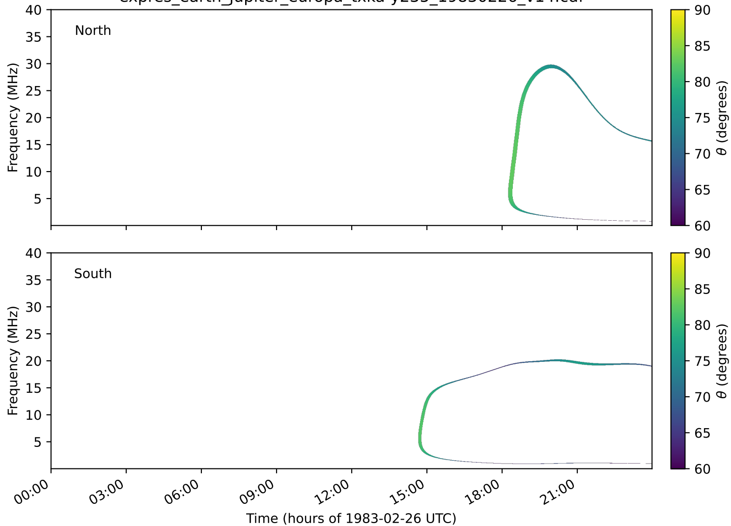
expres_earth_jupiter_europa_txka-y235_19830226_v14.cdf
