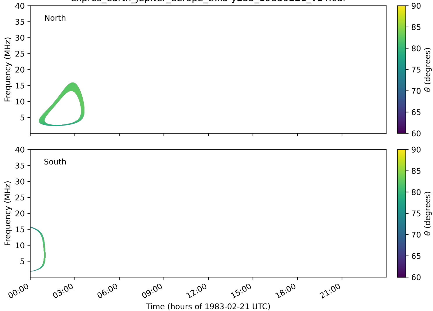
expres_earth_jupiter_europa_txka-y235_19830221_v14.cdf
