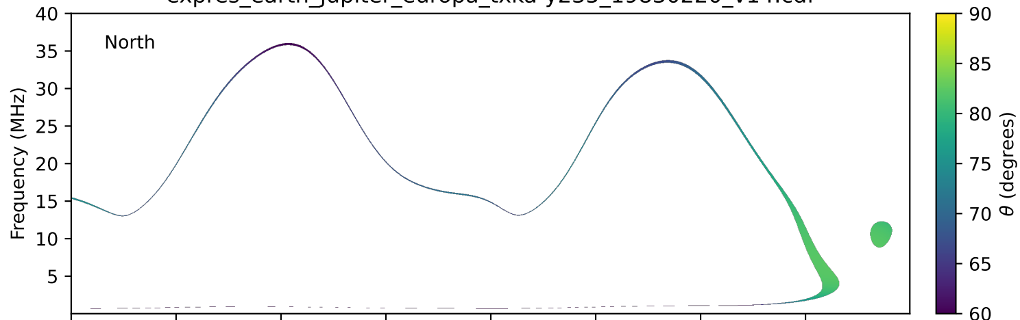
expres_earth_jupiter_europa_txka-y235_19830220_v14.cdf
