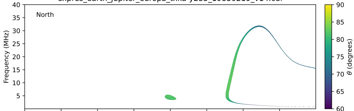
expres_earth_jupiter_europa_txka-y235_19830219_v14.cdf
