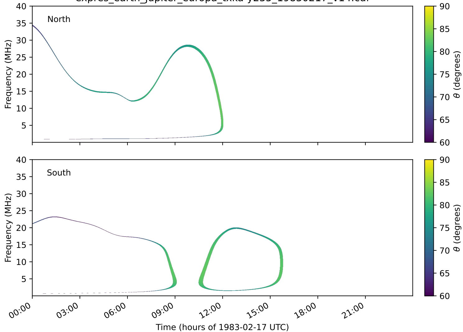
expres_earth_jupiter_europa_txka-y235_19830217_v14.cdf
