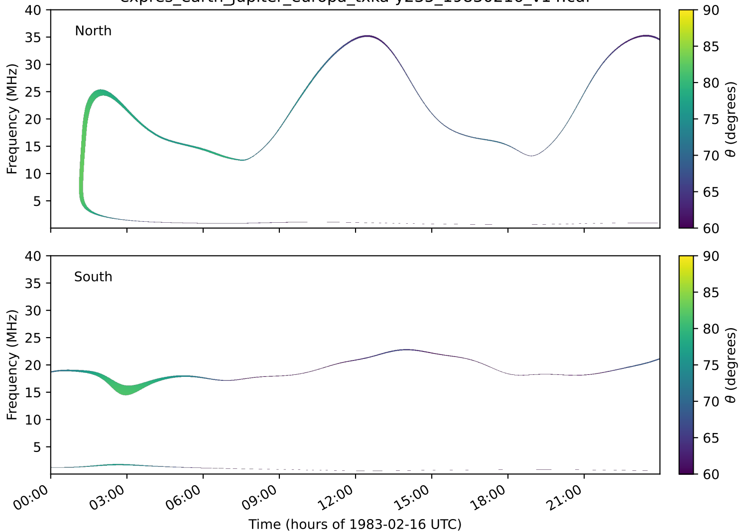
expres_earth_jupiter_europa_txka-y235_19830216_v14.cdf
