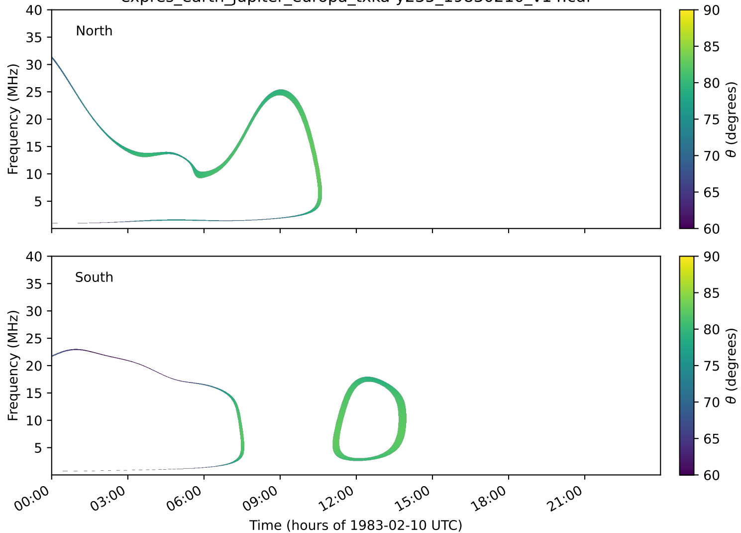
expres_earth_jupiter_europa_txka-y235_19830210_v14.cdf
