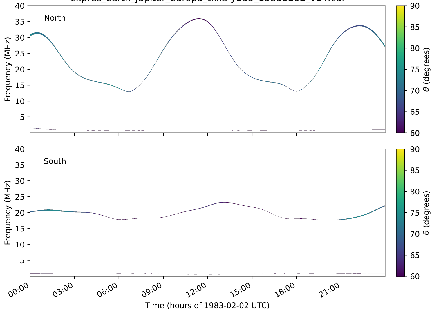
expres_earth_jupiter_europa_txka-y235_19830202_v14.cdf
