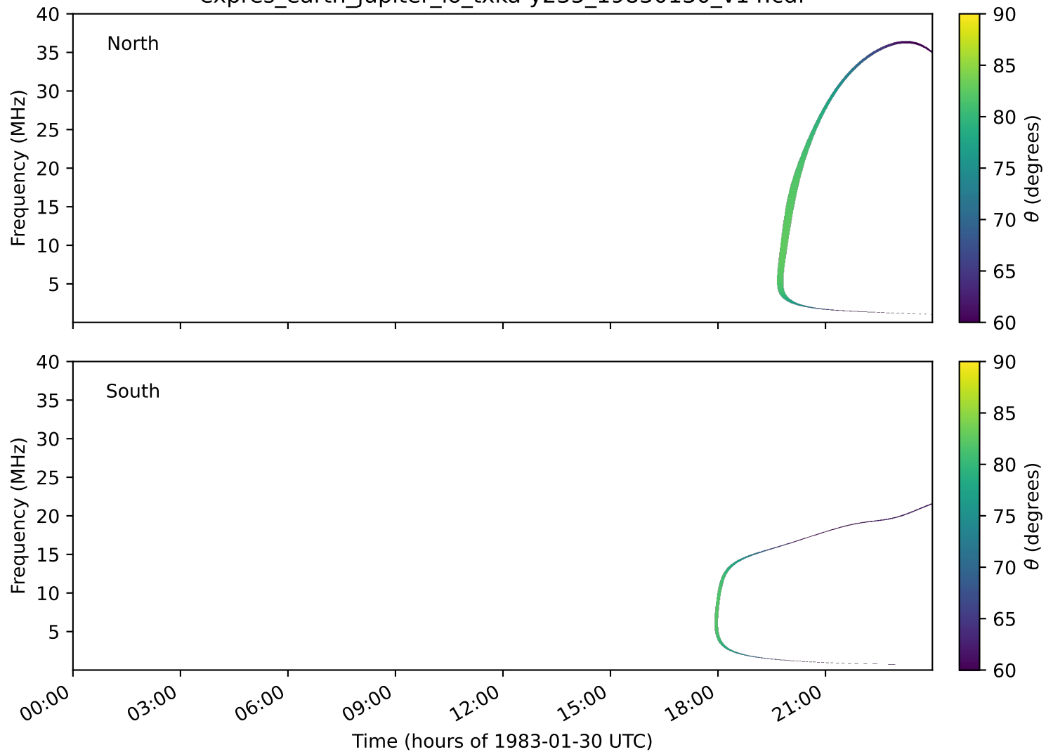
expres_earth_jupiter_io_txka-y235_19830130_v14.cdf
