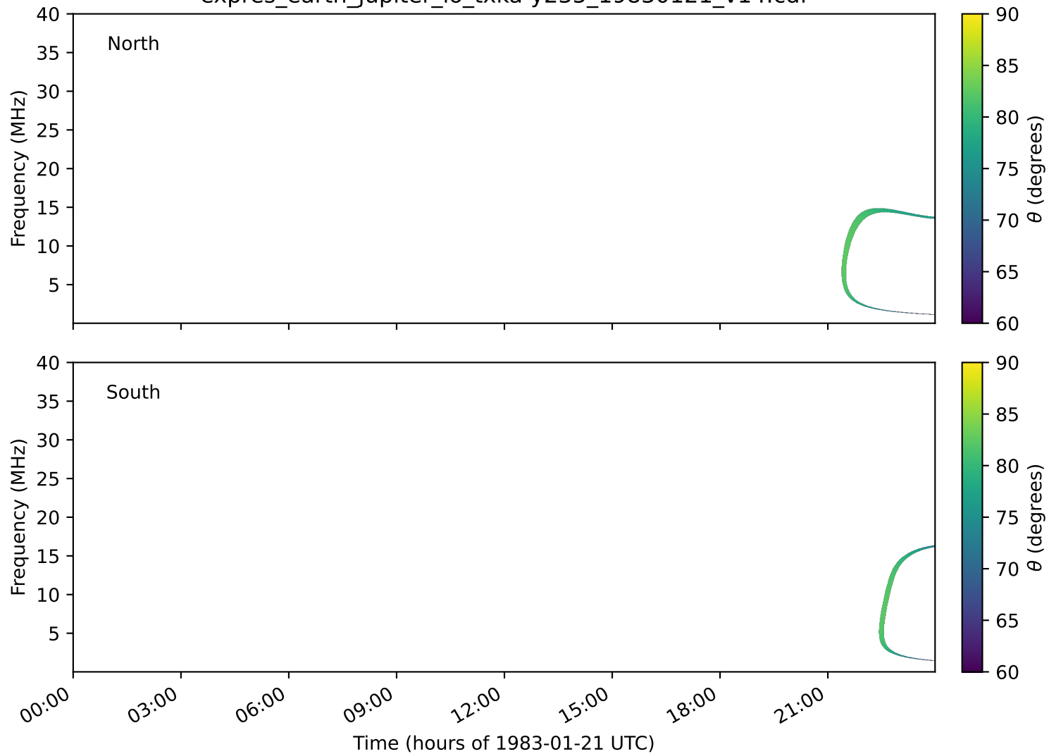
expres_earth_jupiter_io_txka-y235_19830121_v14.cdf
