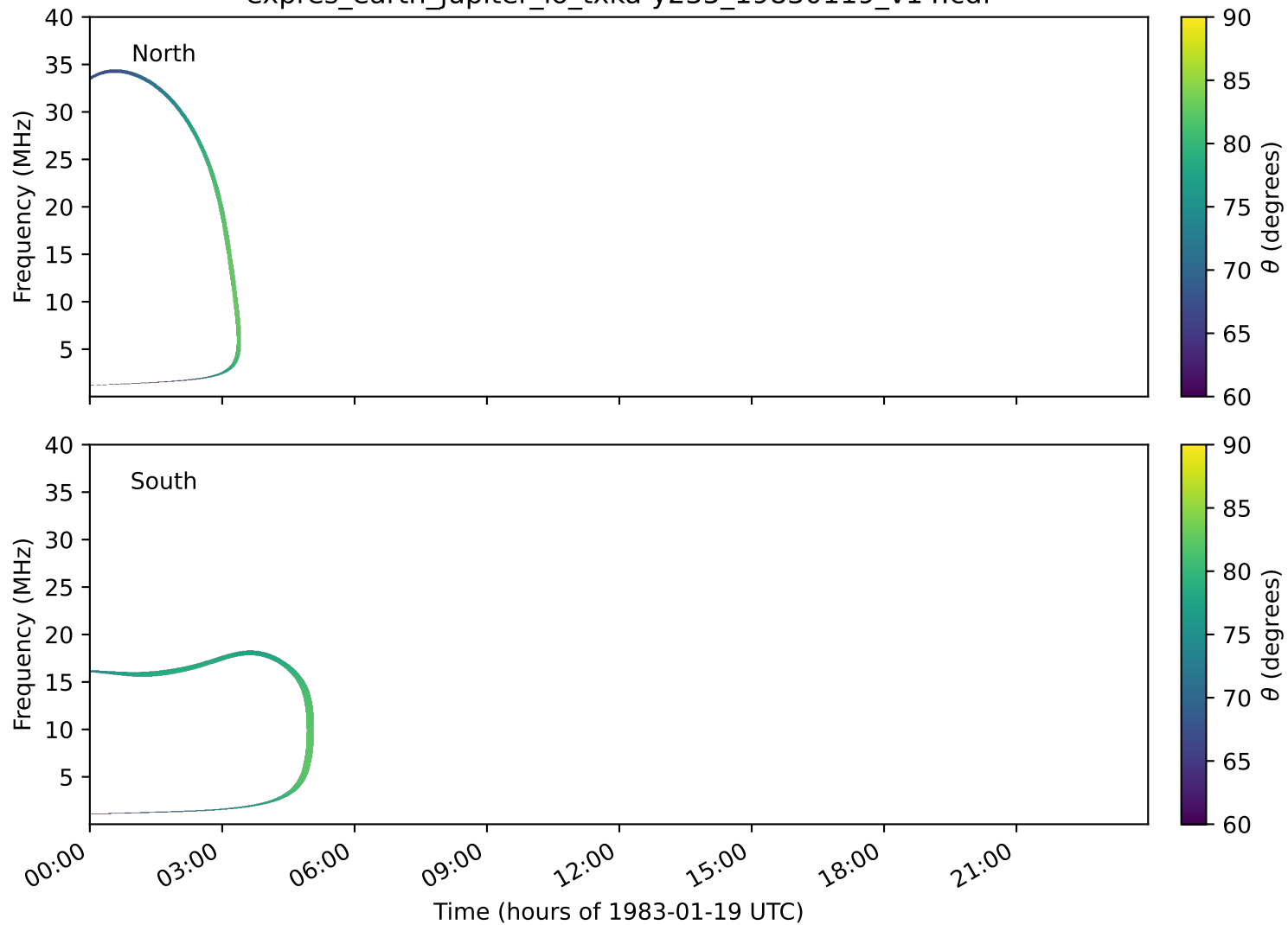
expres_earth_jupiter_io_txka-y235_19830119_v14.cdf
