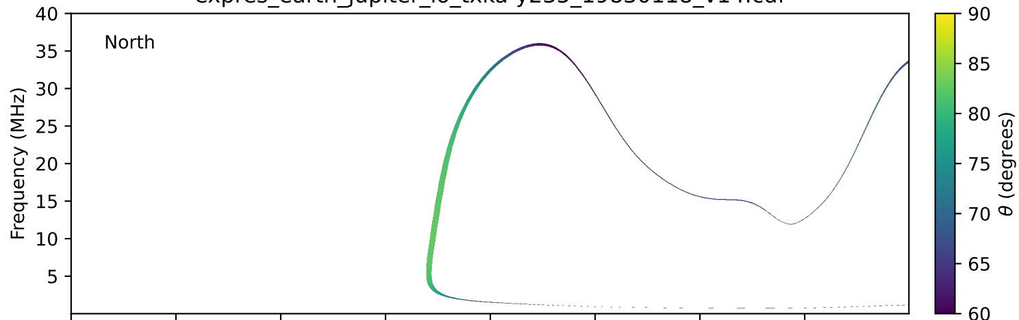
expres_earth_jupiter_io_txka-y235_19830118_v14.cdf
