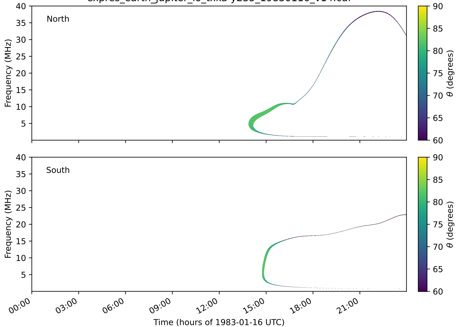
expres_earth_jupiter_io_txka-y235_19830116_v14.cdf
