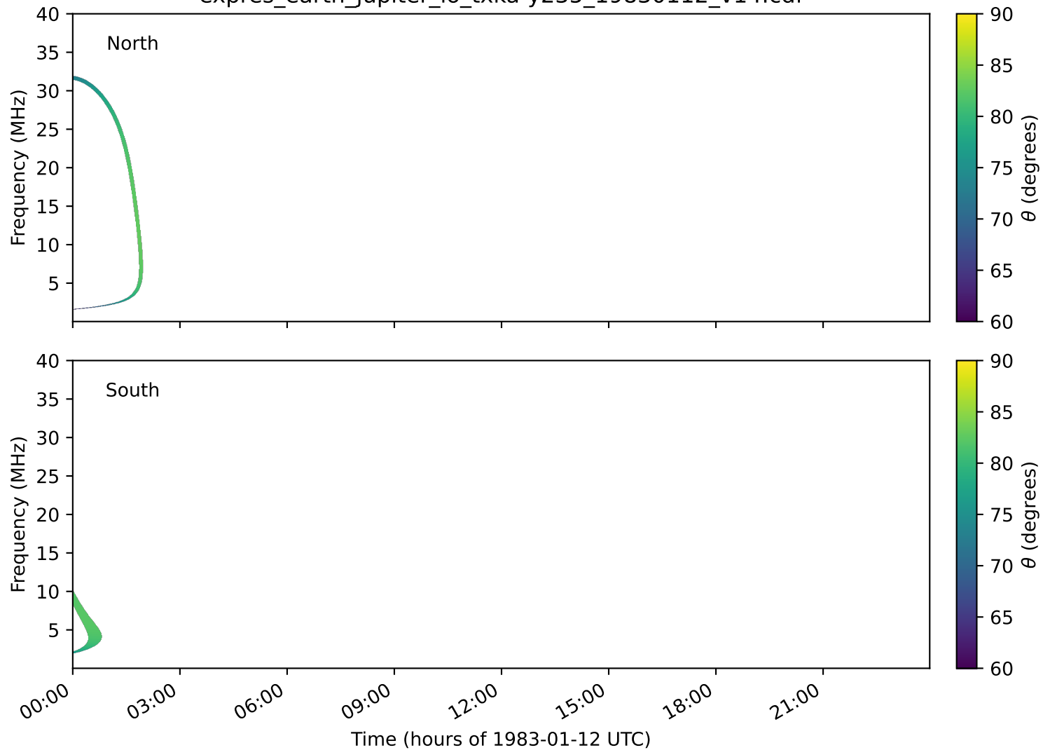
expres_earth_jupiter_io_txka-y235_19830112_v14.cdf
