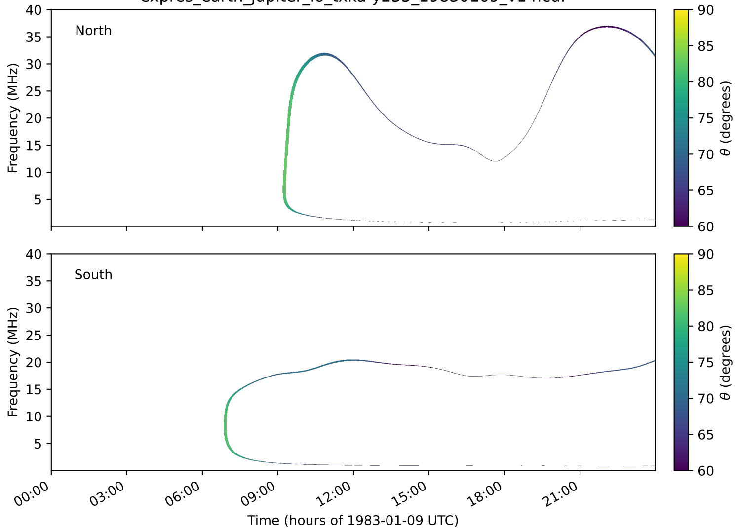
expres_earth_jupiter_io_txka-y235_19830109_v14.cdf
