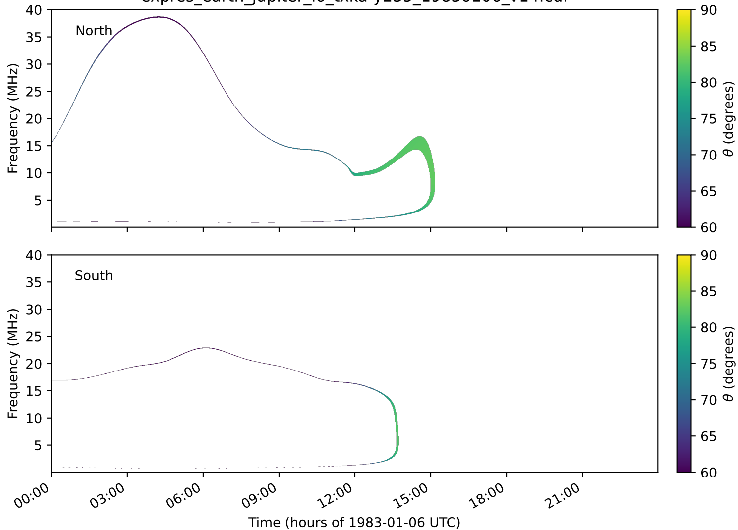
expres_earth_jupiter_io_txka-y235_19830106_v14.cdf
