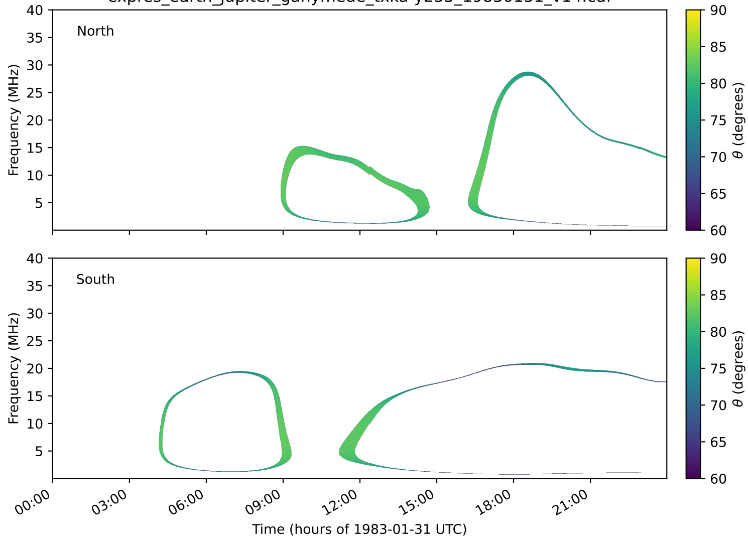
expres_earth_jupiter_ganymede_txka-y235_19830131_v14.cdf
