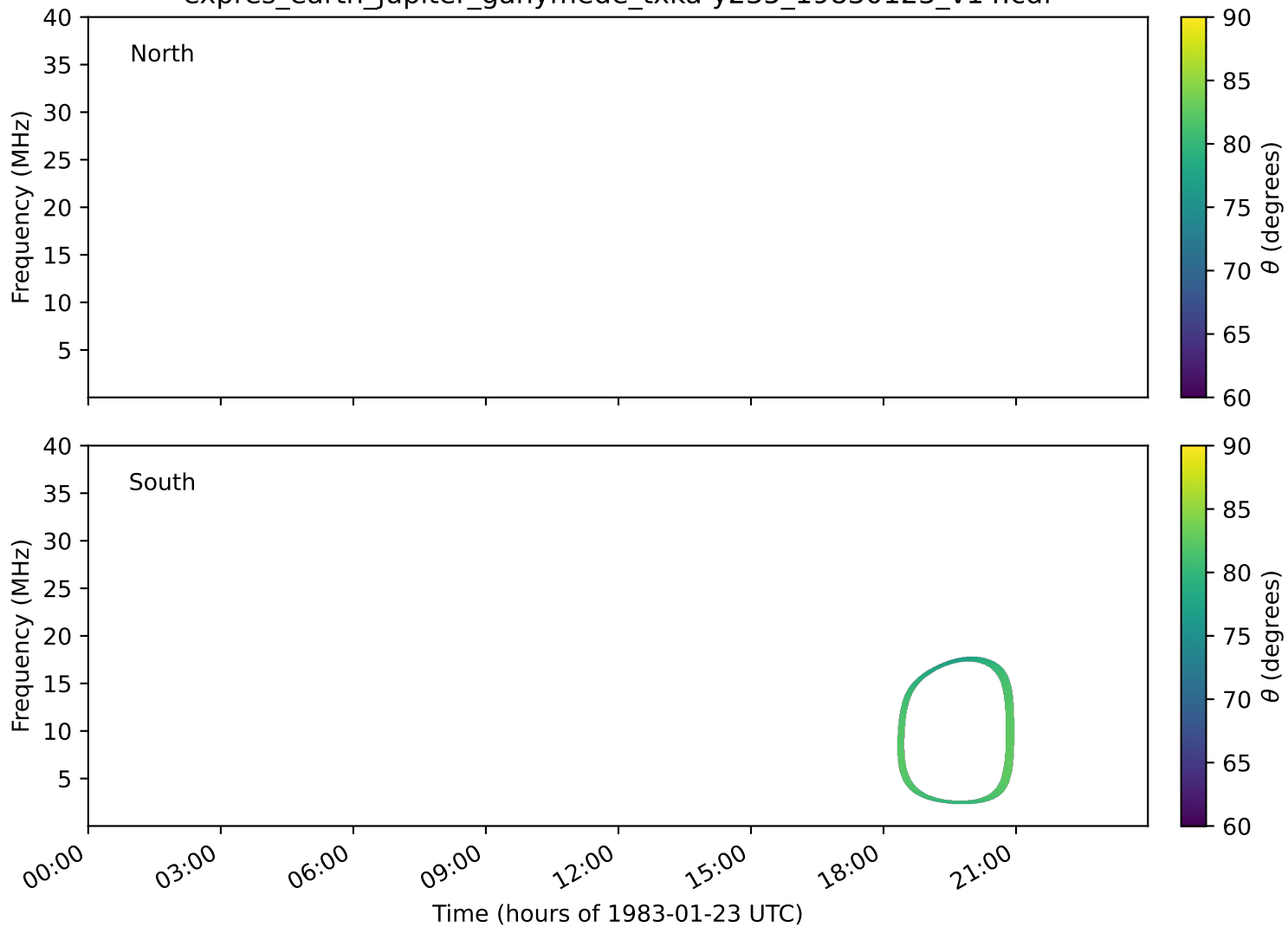
expres_earth_jupiter_ganymede_txka-y235_19830123_v14.cdf
