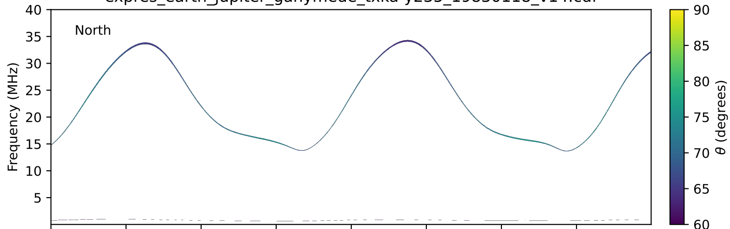
expres_earth_jupiter_ganymede_txka-y235_19830118_v14.cdf
