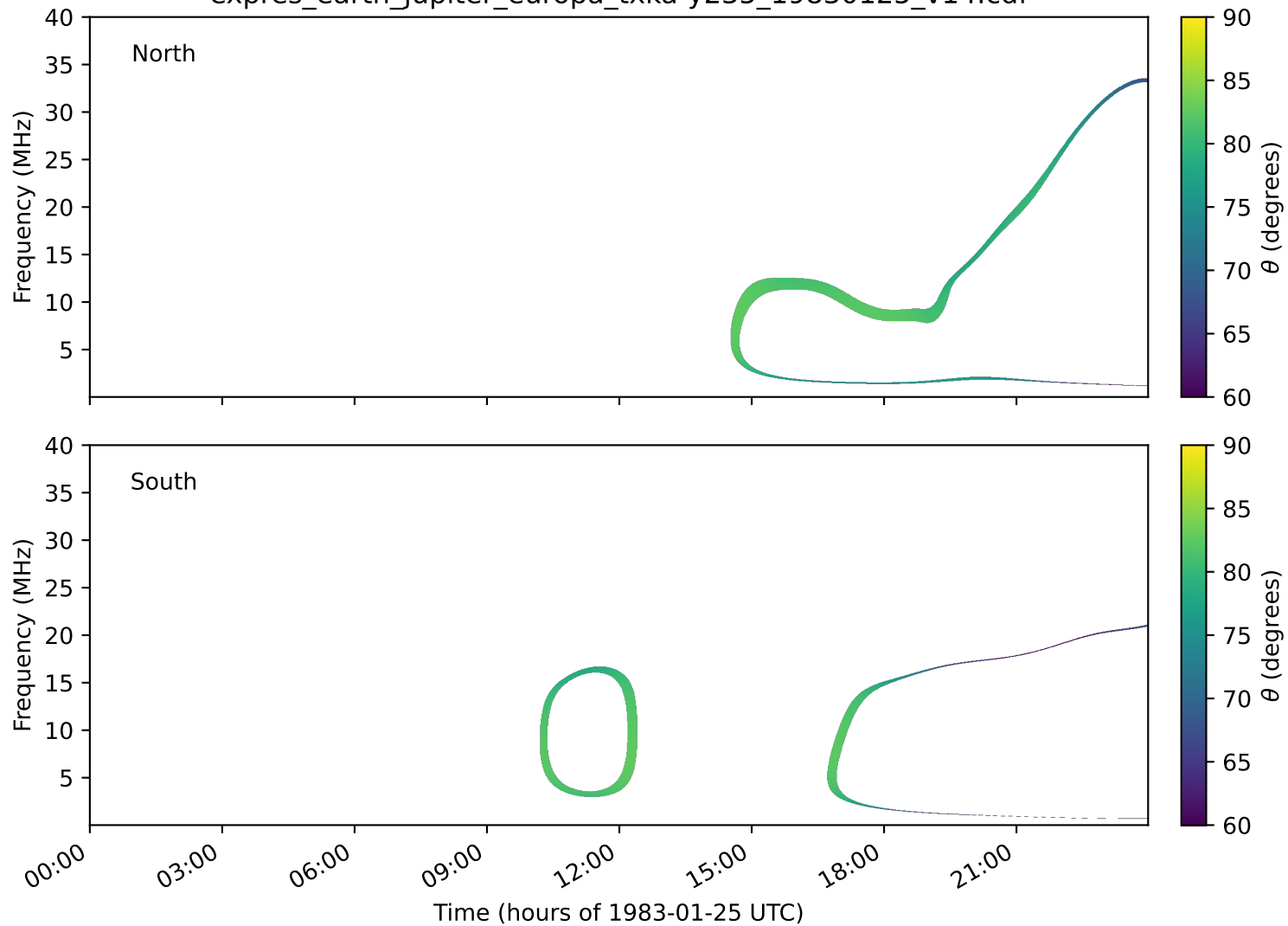
expres_earth_jupiter_europa_txka-y235_19830125_v14.cdf
