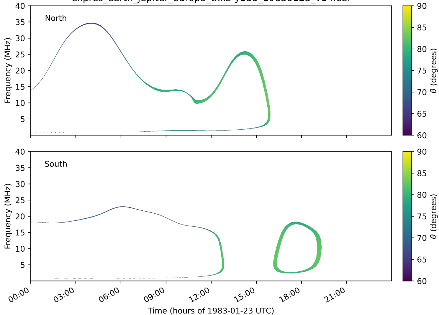
expres_earth_jupiter_europa_txka-y235_19830123_v14.cdf
