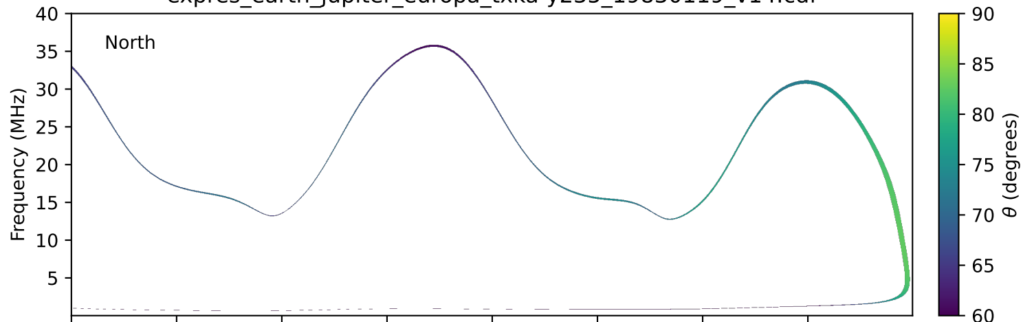
expres_earth_jupiter_europa_txka-y235_19830119_v14.cdf
