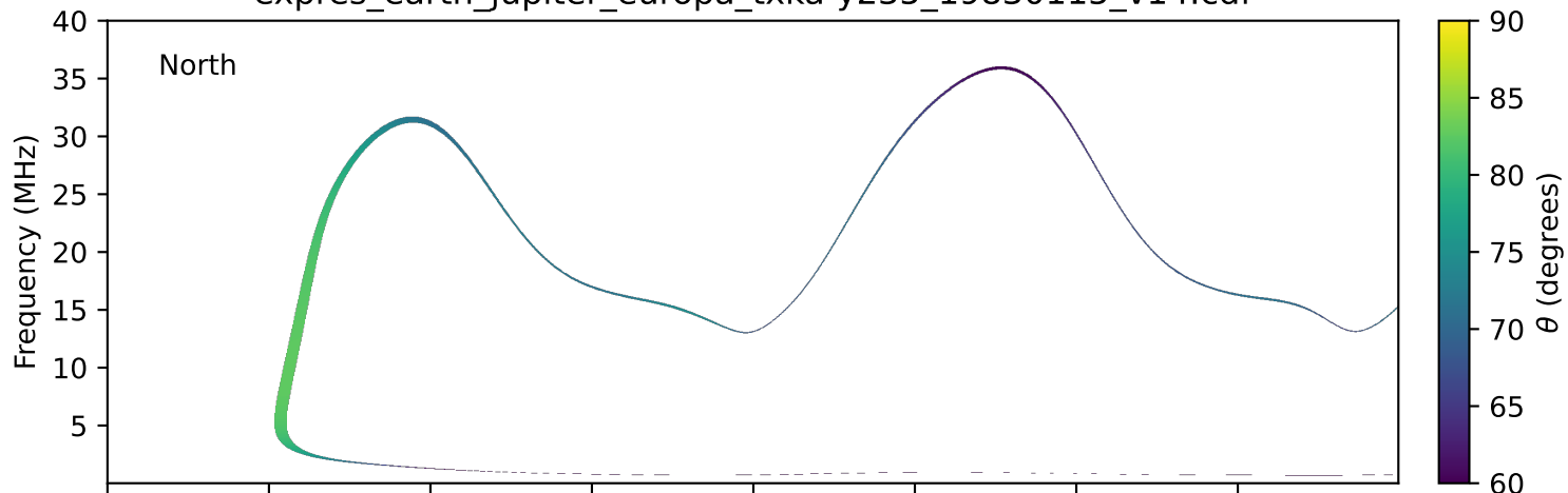
expres_earth_jupiter_europa_txka-y235_19830115_v14.cdf
