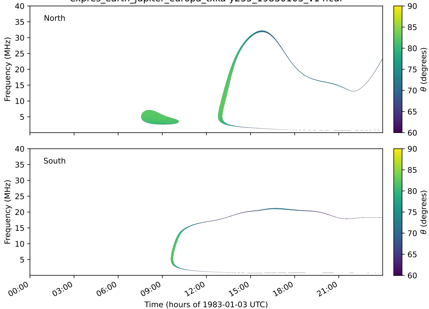
expres_earth_jupiter_europa_txka-y235_19830103_v14.cdf
