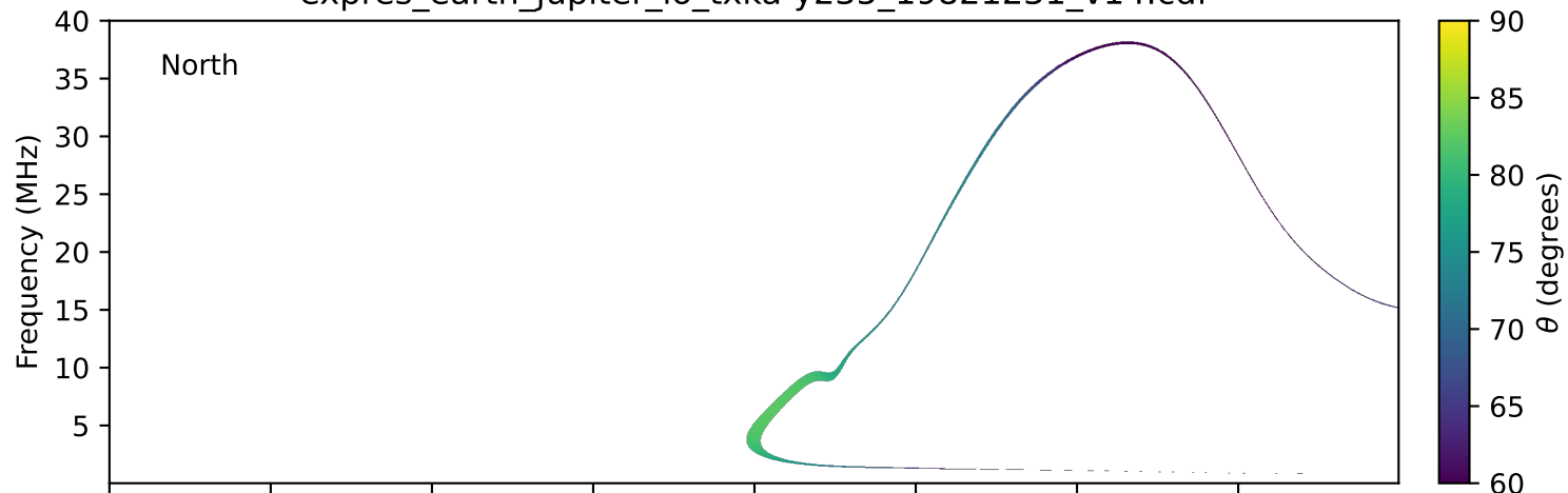
expres_earth_jupiter_io_txka-y235_19821231_v14.cdf
