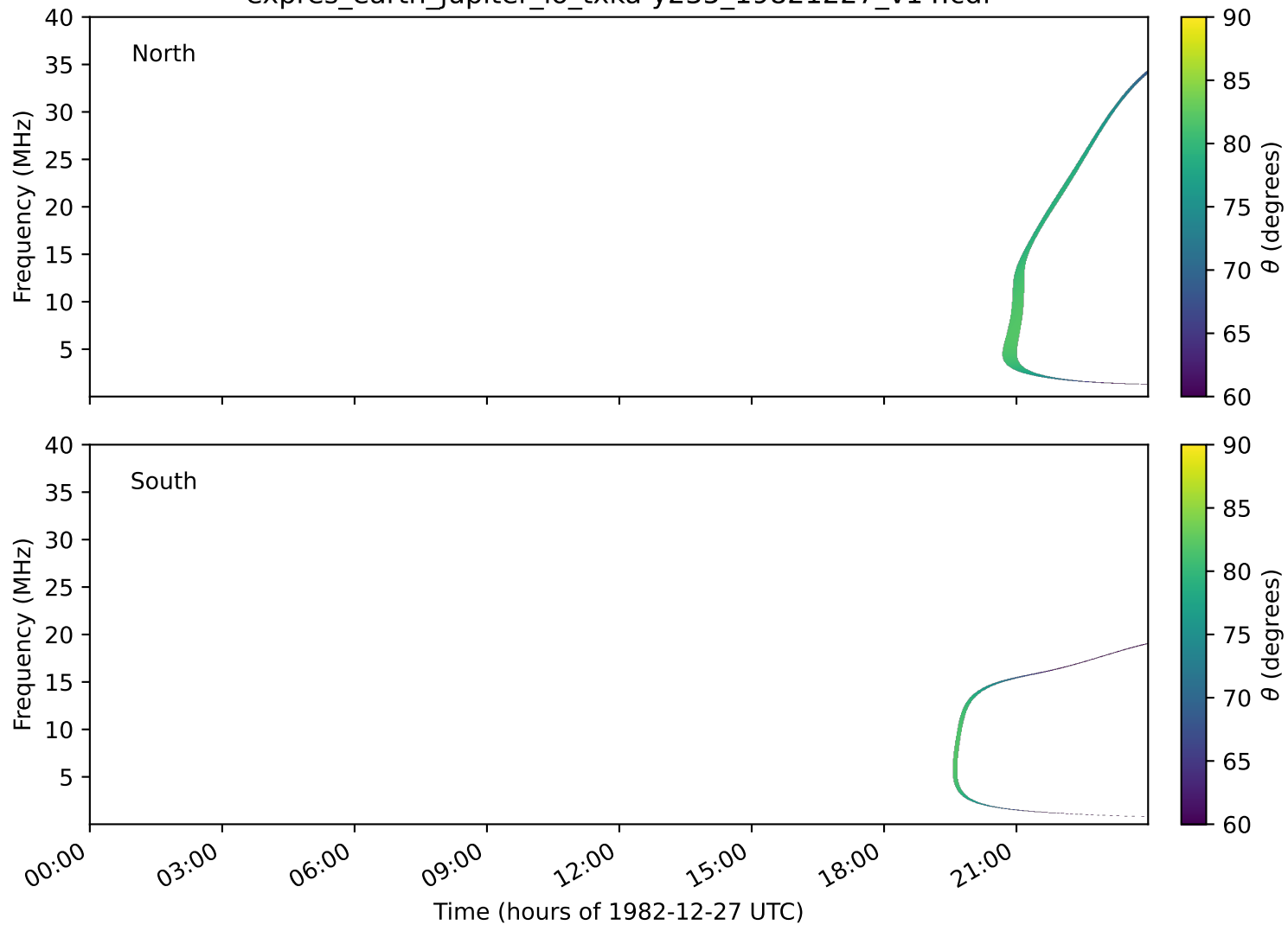
expres_earth_jupiter_io_txka-y235_19821227_v14.cdf
