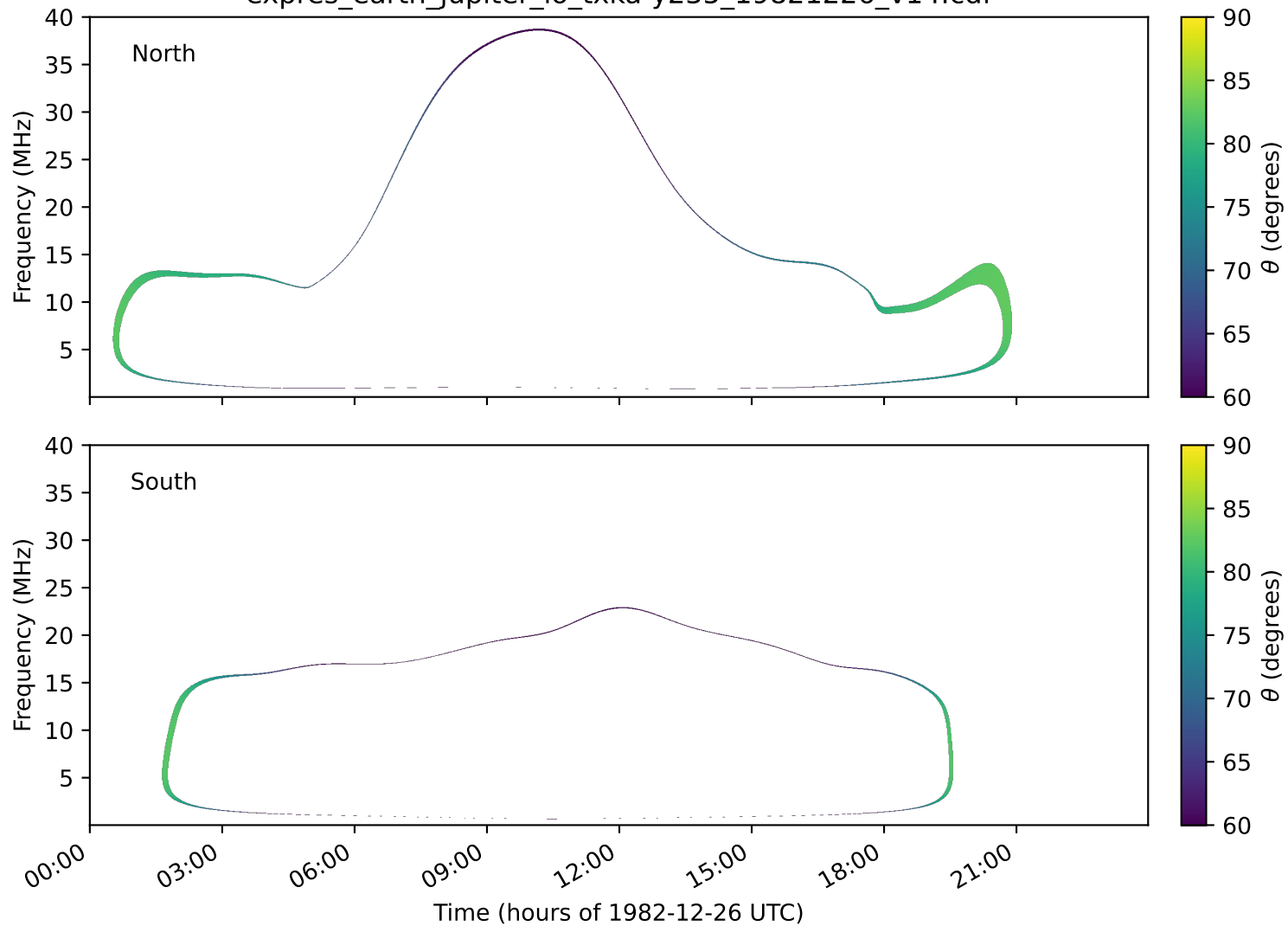
expres_earth_jupiter_io_txka-y235_19821226_v14.cdf
