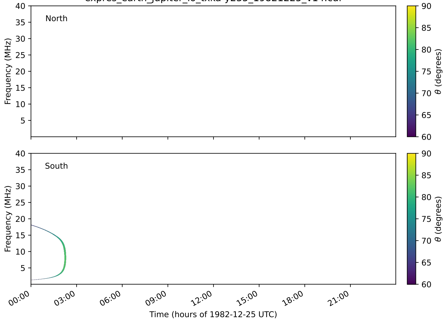
expres_earth_jupiter_io_txka-y235_19821225_v14.cdf
