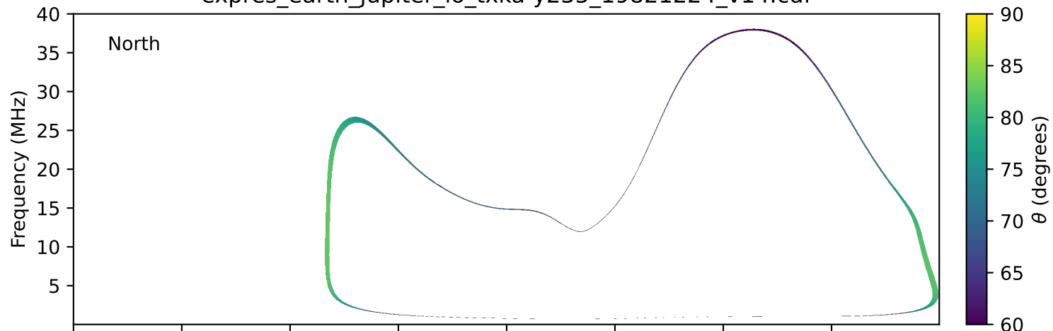
expres_earth_jupiter_io_txka-y235_19821224_v14.cdf
