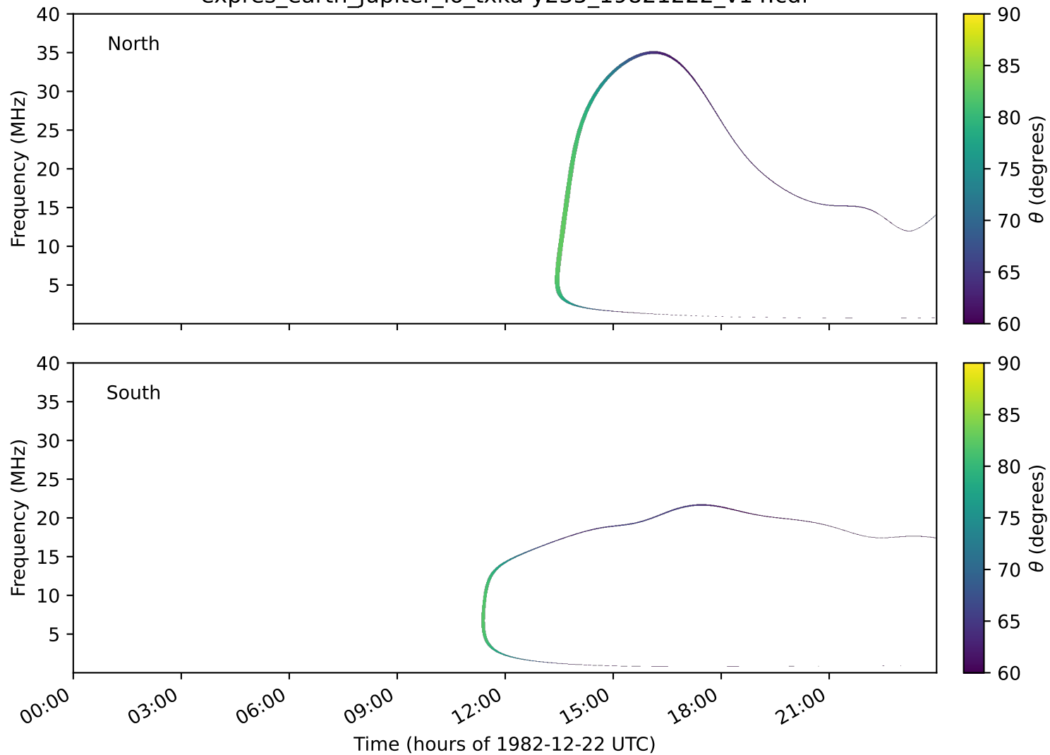
expres_earth_jupiter_io_txka-y235_19821222_v14.cdf
