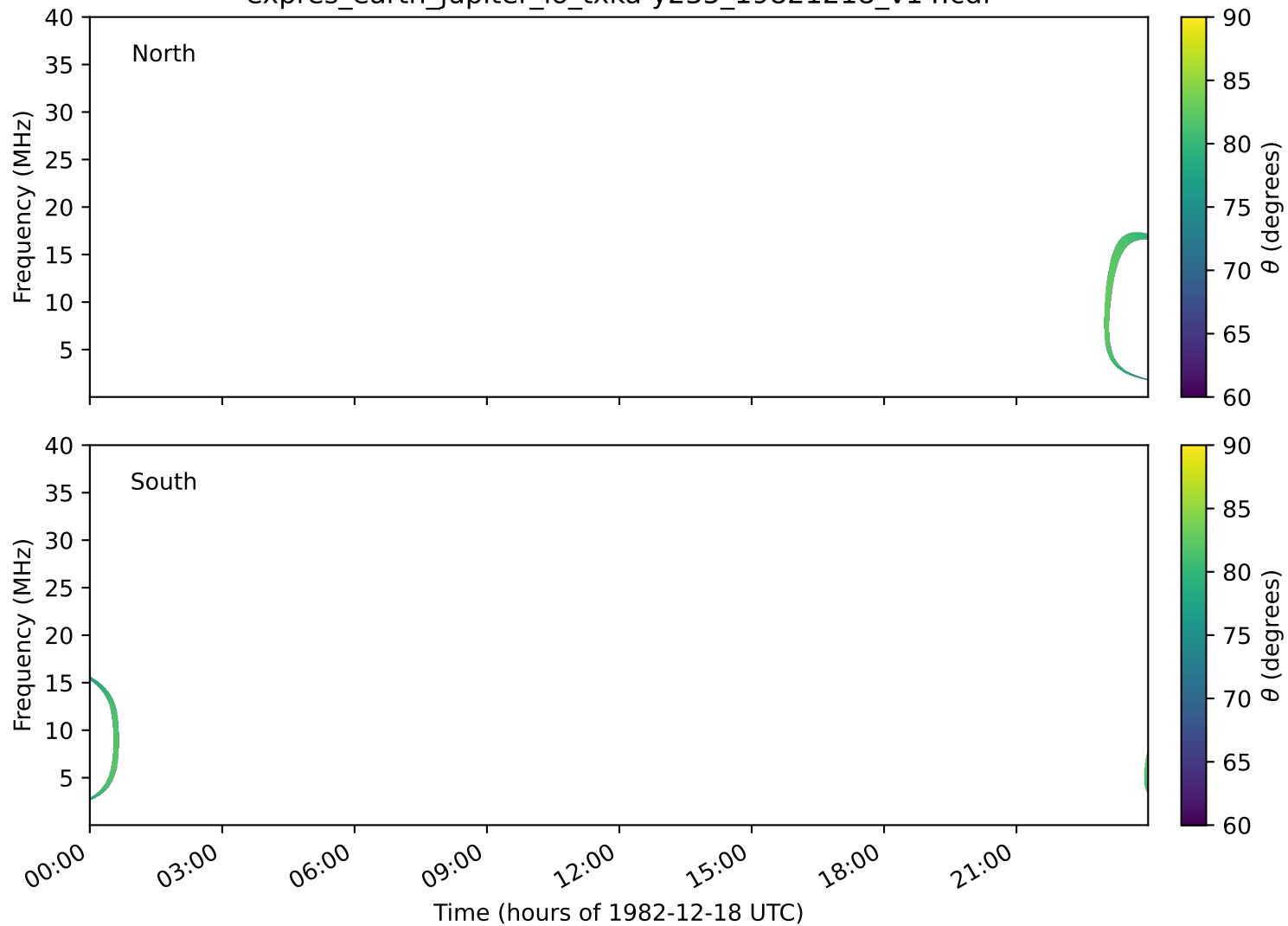
expres_earth_jupiter_io_txka-y235_19821218_v14.cdf
